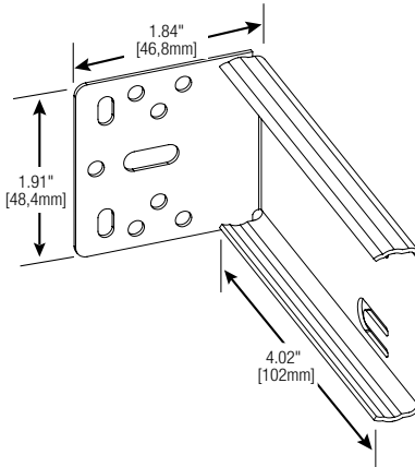
Rear Mounting Bracket (sold separately)
