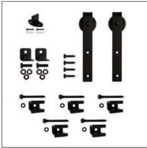
FR-HK-08 3" Hook Carriers Side Mount Black Finish
